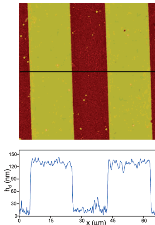
Figure 2. AFM scan ( 70 \times 70 \mu\text{m}^2 ) along with a section analysis of the patterned PS grafts on UNCD. Photopolymerization by UV irradiation ( \lambda_{\text{max}} = 350 nm). Irradiation time: 16 h. Polystyrene layer thickness: 109 \pm 9 nm. The native UNCD regions have a roughness of 9.6 nm rms, the PS coated regions of 6.0 nm rms.
